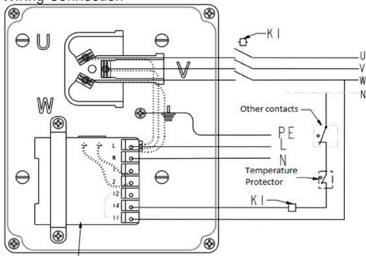
wiring connection
