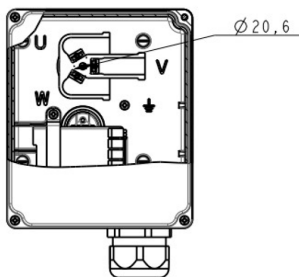
wiring connection
